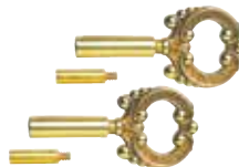
70160 2 Socket Keys Brass Finish With 1/2" Extensions Tapped 3/16"-F x 3/16"-M
